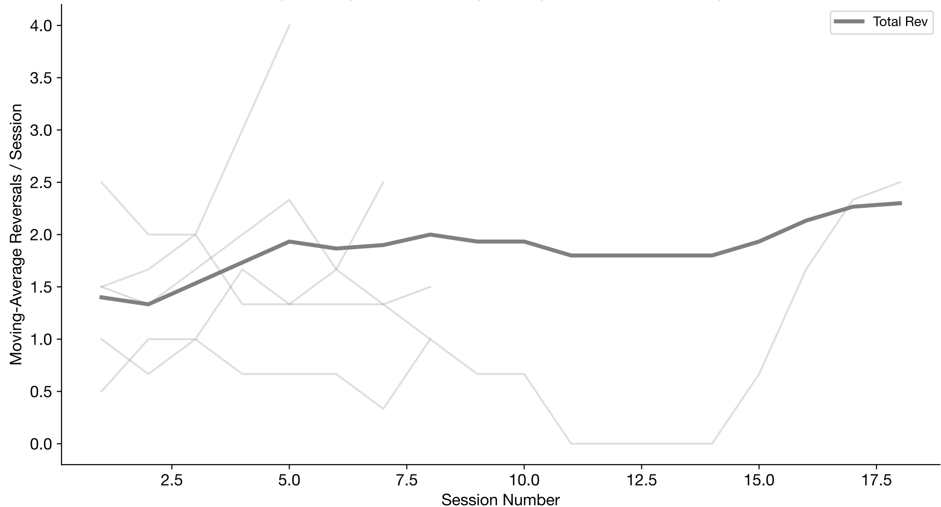
Moving-Average Total Reversals Over Time (n=5 subjects; sessions per subject=5–18; window=3)
